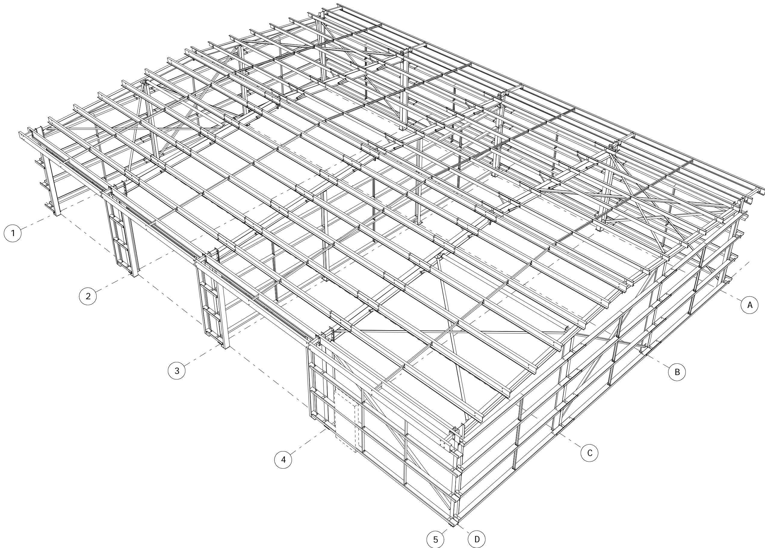
3-D VIEW
